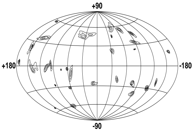
Fig. 4. Statistical (1-, 2-, and 3-sigma) location contours, in Galactic coordinates, of 29 gamma-ray bursts observed through viewing period 419.5. The extent of the contours depends on the strength of the burst (from Kippen et al. 1998a)
