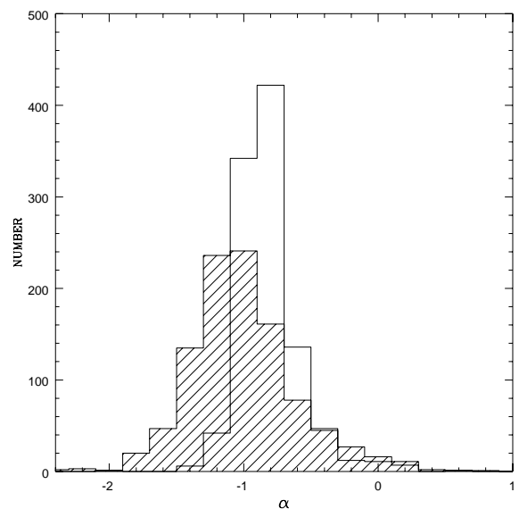
Fig. 2. Histogram of low ( \alpha_l )- and high-frequency ( \alpha_h ) spectral indices. The blank area corresponds to \alpha_l , the hashed one to \alpha_h
