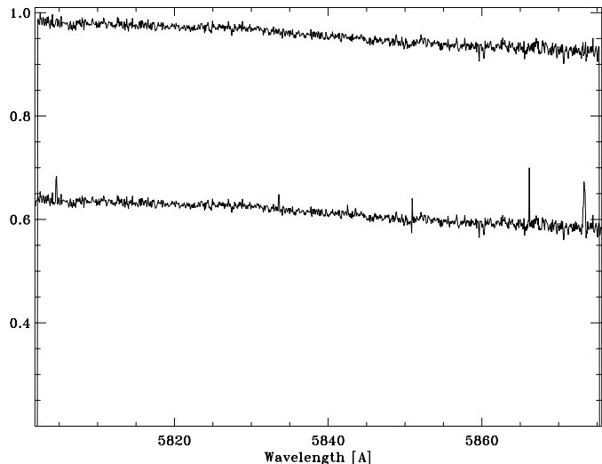
Fig. 9. Difference between the results of RAW_ORDER and OPT_EXTR demonstrating essentially the removal of cosmic events. The two spectra are offset by a constant amount
