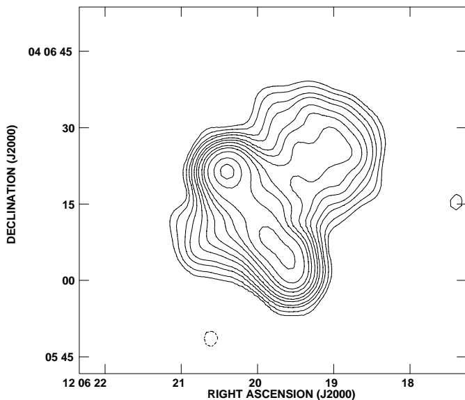
Fig. 10. VLA image of 1203+043 at 320 MHz. Contours are at -5, 5, 10, 20, 30, 50, 70, 100, 150, 200, 300, 500, 700, 800 \text{mJy beam}^{-1} . The peak flux density is 796 \text{ mJy beam}^{-1}
