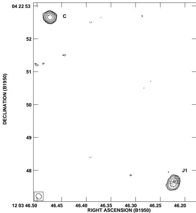
Fig. 9. VLA image of 1203+043 at 15 GHz. Contours are at -0.4, 0.4, 0.6, 1, 2, 4, 8, 16, 32 \text{mJy beam}^{-1} . The peak flux density is 14.5 \text{ mJy beam}^{-1} . A vector length of 1'' = 10 \text{ mJy beam}^{-1}
