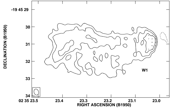
Fig. 3. VLA image of the West lobe of 0235–197 at 8.4 GHz. Contours are at -0.3, 0.3, 0.6, 1, 2, 4, 8, 16, 32, 64 mJy beam ^{-1} . A vector length of 1'' = 10 mJy beam ^{-1}
