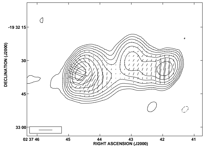
Fig. 4. VLA image of the East lobe of 0235–197 at 15 GHz. Contours are at -0.4, 0.4, 0.6, 1, 2, 4, 6, 10, 15, 20 mJy beam ^{-1} . The peak flux density is 15.7 mJy beam ^{-1} . A vector length of 1'' = 6.7 mJy beam ^{-1}
