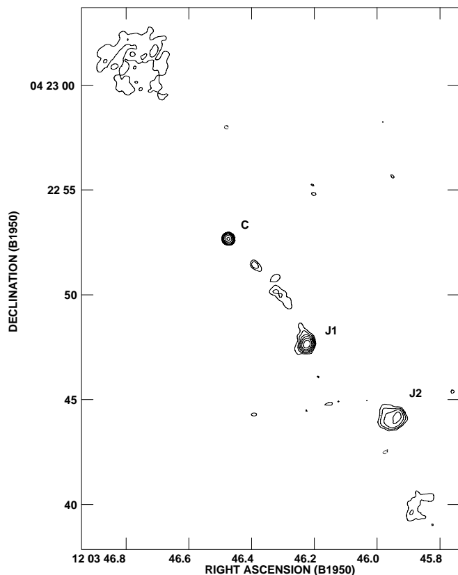
Fig. 7. VLA image of 1203+043 at 8.4 GHz. Contours are at -0.25, 0.25, 0.5, 1, 2, 4, 8, 16, 32, 64, 128 \text{mJy beam}^{-1} . The peak flux density is 14.8 \text{ mJy beam}^{-1} .
