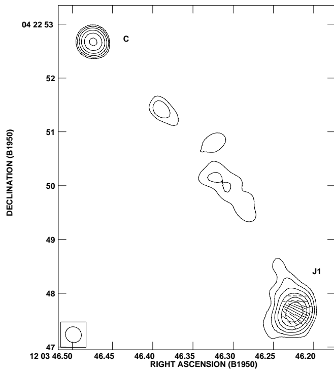
Fig. 8. VLA image of the central region of 1203+043 at 8.4 GHz. Contours are at -0.25, 0.25, 0.5, 1, 2, 4, 8, 16, 32, 64, 128 \text{mJy beam}^{-1} . The peak flux density is 14.8 \text{ mJy beam}^{-1} . A vector length of 1'' = 10 \text{ mJy beam}^{-1} .
