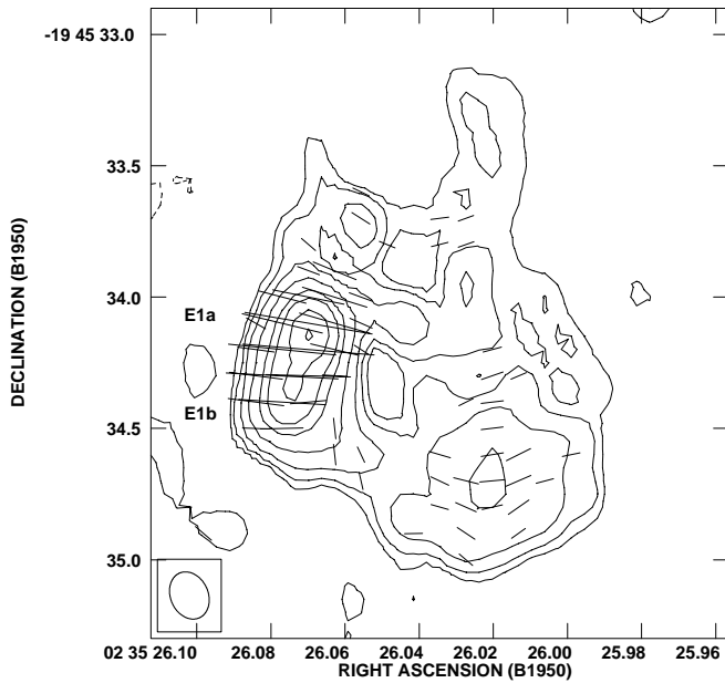
Fig. 5. VLA image of 0235–197 at 320 MHz. Contours are at -5, 5, 10, 20, 50, 100, 150, 200, 300, 500, 700, 1000, 1500, 2000, 2500 mJy beam ^{-1} . The peak flux density is 3430 mJy beam ^{-1}
