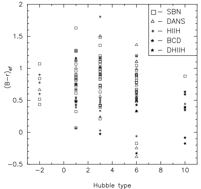
Fig. 4. Relation between spectroscopic and morphological types and (B-r)_{ef} colour. We have selected the main spectroscopic types of our sample: SBN, DANS, HIII and BCD & DIIIH, as classified in Gallego et al. (1996) and morphological types from S0 to Irr; the galaxies classified as Sc+ by Vitores et al. (1996a) are included in T = 6 -corresponding to a Sc galaxy
